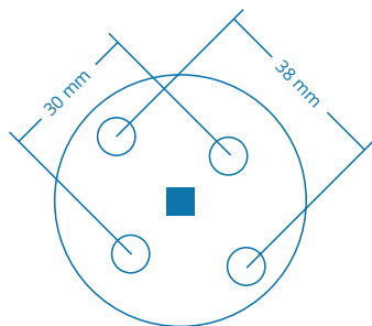
Universaalne kinnitus 38mm / 30mm
